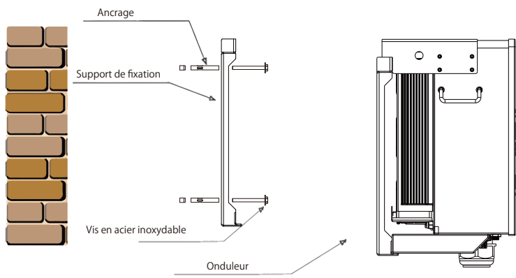
Pic 4.5 Inverter Installation
