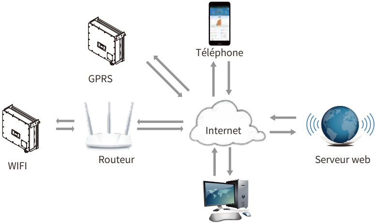
Image 5.13 Solution de surveillance via Internet
