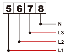
Charge (5, 6, 7, 8)
