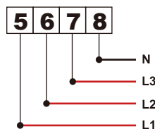
Charge (5, 6, 7, 8)
