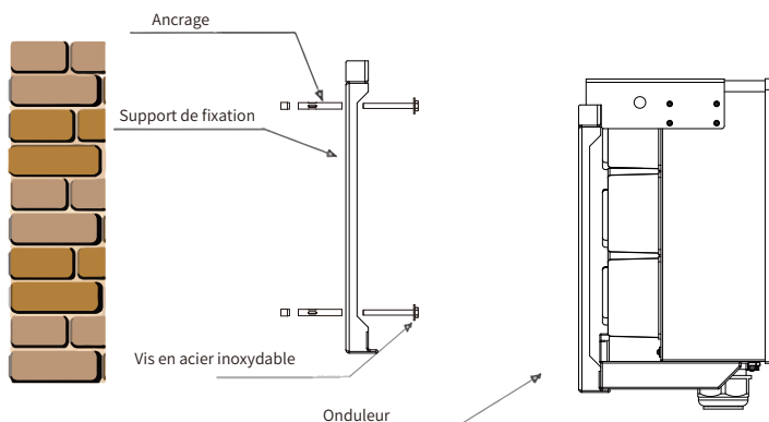
Pic 4.5 Inverter Installation
