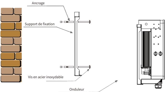
Pic 4.5 Inverter Installation
